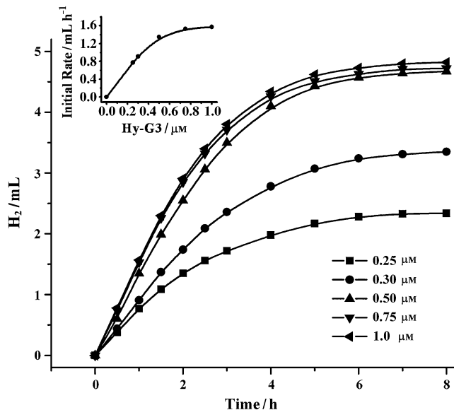
Figure 4. Photocatalytic evolution of H 2 in acetone/H 2 O=9:1 with different concentrations of Hy-G3. Hydrogen production was calculated on the basis of the amount of hydrogen generated in 10 mL of the sample solution over 8 h irradiation (16 mWcm -2 ). [Ir(ppy) 2 (bpy)PF 6 ]=5 × 10 -4 M, [TEA]=0.6 M, [Hy-G3]=0.25–1.0 μM. Inset: Initial rate of hydrogen evolution versus [Hy-G3].
